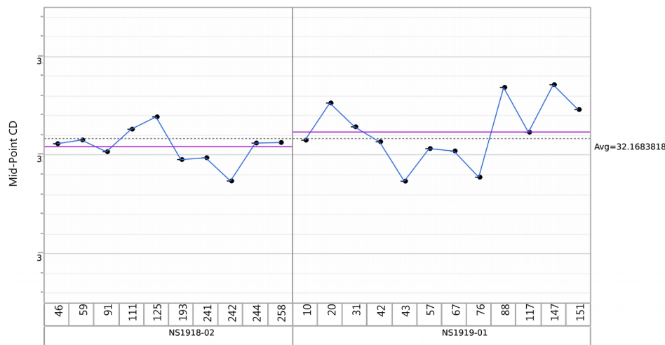
Figure 2. Initial CD Repeatability (2 Stamps, Same Master)
